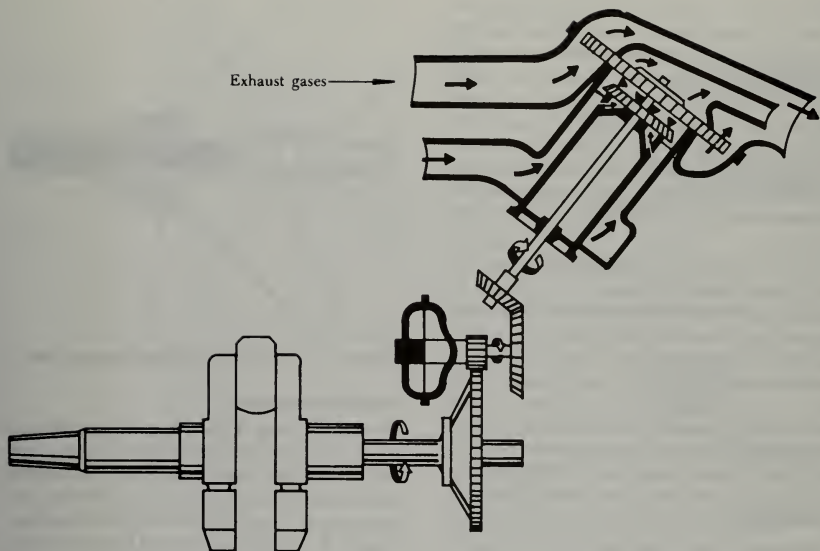
FIGURE 2-17. Transmission of turbine power to crankshaft.
